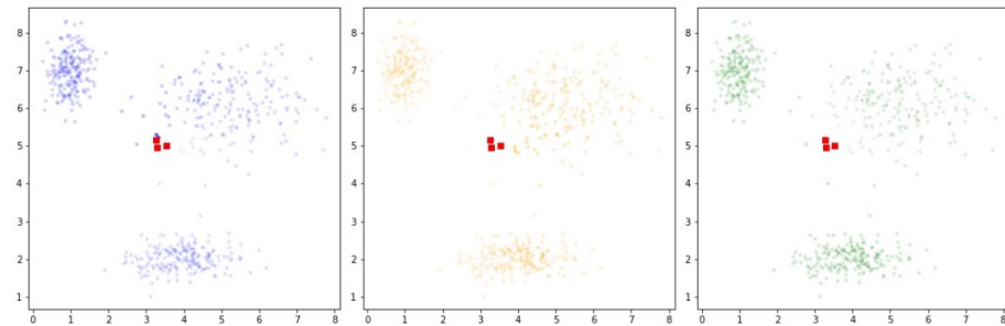
Iteration 1
