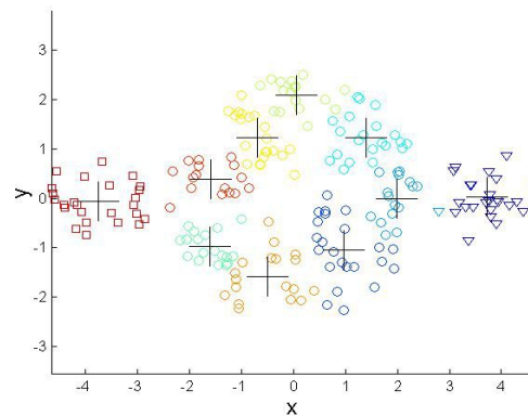
K-means (10 Clusters)
