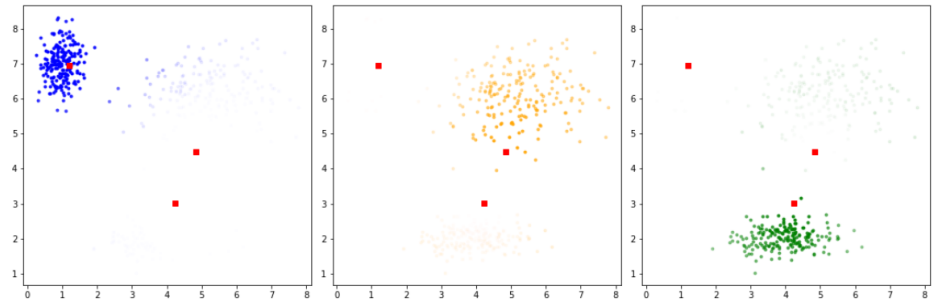
Iteration 6
