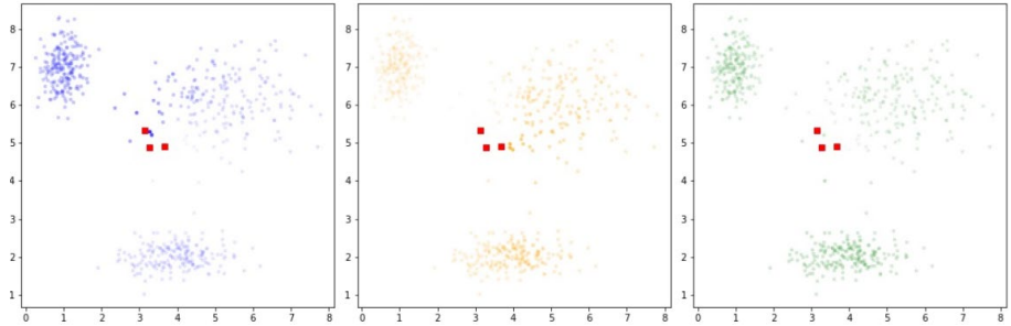
Iteration 2
