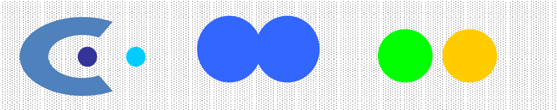
6 density-based clusters
