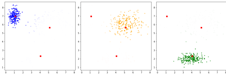
Iteration 7
