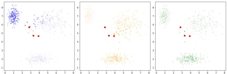
Iteration 3
