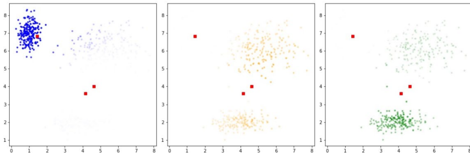
Iteration 5
