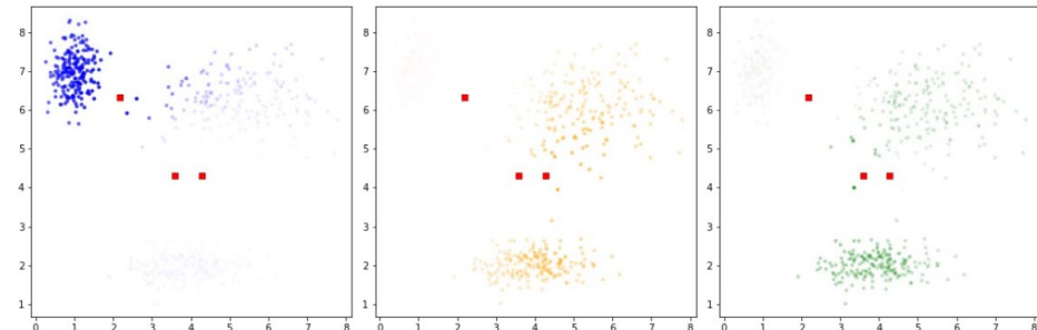
Iteration 4
