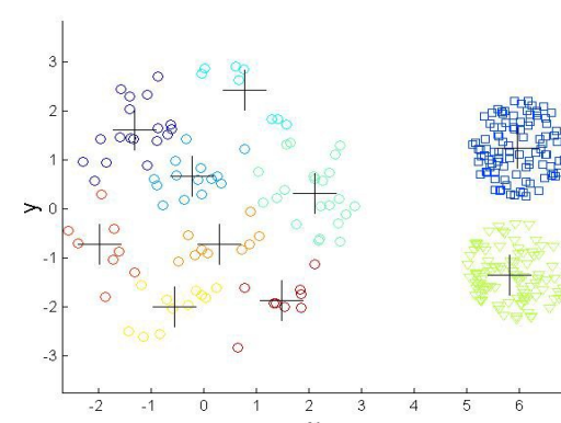
K-means (10 Clusters)
