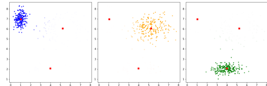
Iteration 8
