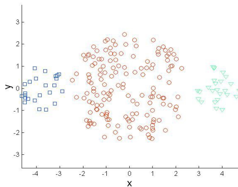
Original Points
