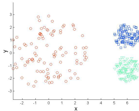
Original Points
